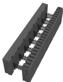
VV26 RADONBLOKK STANDARD H300 X L1200 X B350
